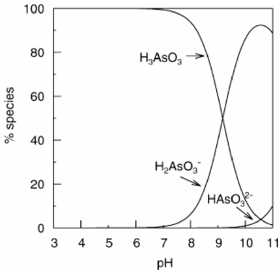
Figure 1.1: Arsenite speciation as a function of pH – ionic strength of about 0.01 mol L -1 (Smedley and Kinniburgh, 2002).
