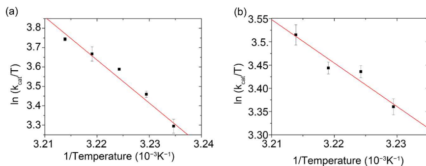
Figure 2. Eyring linear analysis of catalytic constants obtained in different temperatures. Analysis performed at five temperatures for ACh and four for ATCh and adjusted to Eyring equation, Equation (5), where is possible to obtain the thermodynamic parameters of activation, \Delta^\ddagger H and \Delta^\ddagger S . The graph (A) represents the linear regression for ACh and has a correlation coefficient, r = -0.9926 . In (B) is the setting for ATCh with r = -0.9747 .
