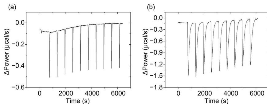
Figure 1. Enthalpy energy obtained from ITC for both substrates. In (a) there is the isothermal curve for ACh. The standard enthalpy was obtained using 4 mM of ACh, in two different injections protocols in the same experiment. The system was allowed to reach thermal equilibrium at 37°C. After a 120 s after the equilibrium period, successive injections of 8 \mu l of 40.0 mM ACh were made every 10 min. The enthalpy was calculated by Equation (3) and a baseline corresponding to heat of dilution was subtracted from the data, and correct to the concentration of AChE 30.0 pM. In (b) the isothermal curve for ATCh 10.0 mM in a protocol only with 8 \mu L injections by the syringe and titrating them in the cell containing 30.0 pM of AChE, with buffer.
