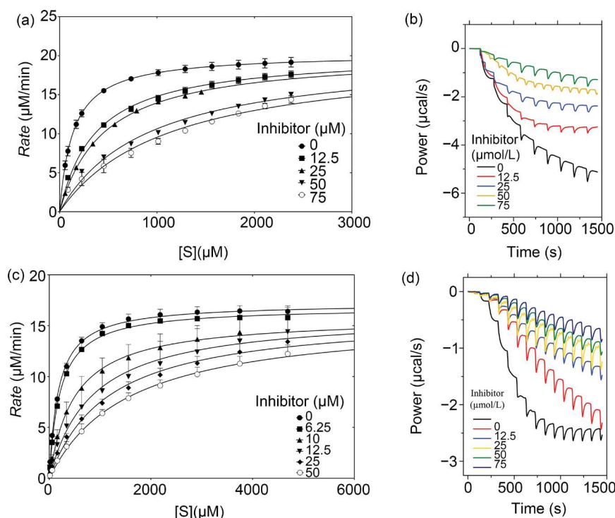
Figure 3. Nonlinear regression analysis of M-M Equation (4) for substrates ACh and ATCh. Kinetic graphs at 310.15 K in the presence and absence of inhibitor aside their ITC graphs. In (a) SNLR for M-M equation for ACh, (b) ITC assays for ACh, (c) SNLR of M-M equation for ATCh, and (d) ITC assays for ATCh. The concentration of inhibitor is \mu\text{mol/L} . Calorimetric assays were performed with successive injections spaced at 150 s between them, containing increasing volumes of 1, 2, 4, 6, and 8 \mu\text{l} until finishing, 20 mM ACh or ATCh, after the equipment has reached thermal equilibrium at 37°C. The change in thermal power was acquired from the baseline shift, transformed to rate using equation (2). The rate was further used to obtain kinetics values through MM-equation, Equation 4. The SNLR analysis was performed concomitantly, resulting in a K_i value, as well the K_m and k_{\text{cat}} .
